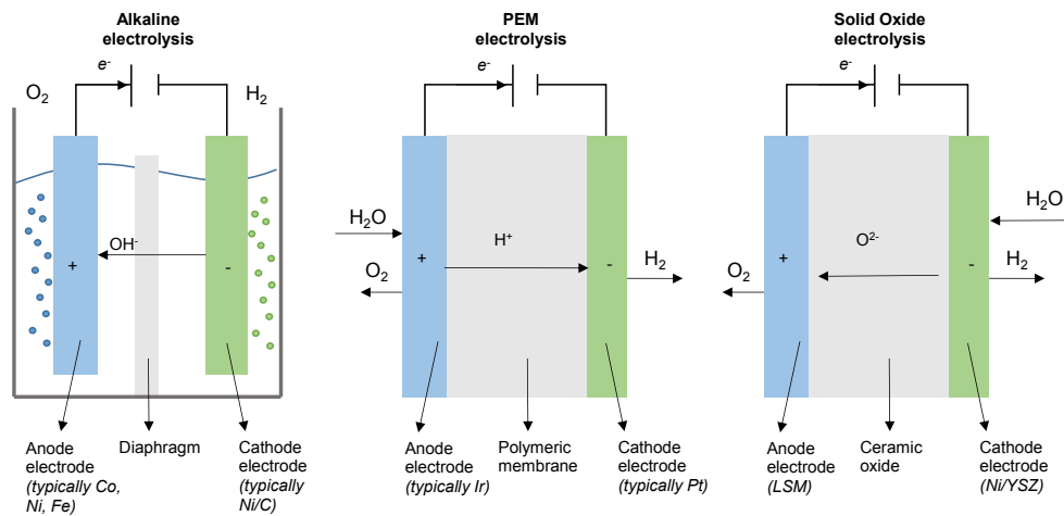
Exhibit 21: Simplified schematic of the three electrolysis technologies for the production of 'green' hydrogen
