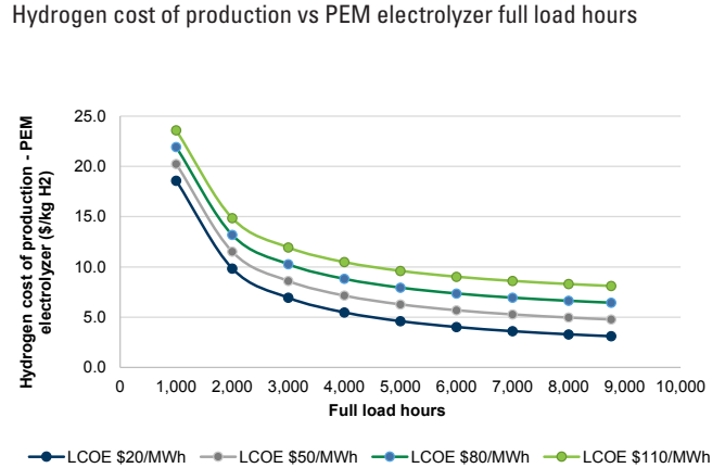
Exhibit 28: ...with a similar trend observed for the PEM electrolyzers
