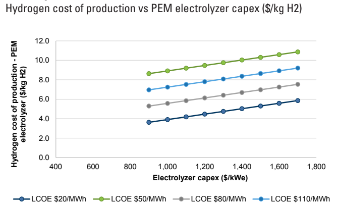
Exhibit 30: ...and a similar trend is observed in more costly PEM electrolyzers
