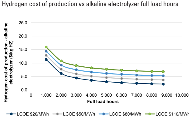
Exhibit 27: The full load hours of the electrolyzer can have a notable impact on the cost of production if <5,000, but cost of production becomes flatter after that for alkaline electrolyzers...
