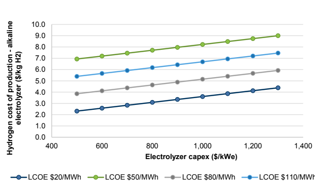
Exhibit 29: The cost of production of 'green' hydrogen shows a linear correlation with electrolyzer capex for alkaline systems...
