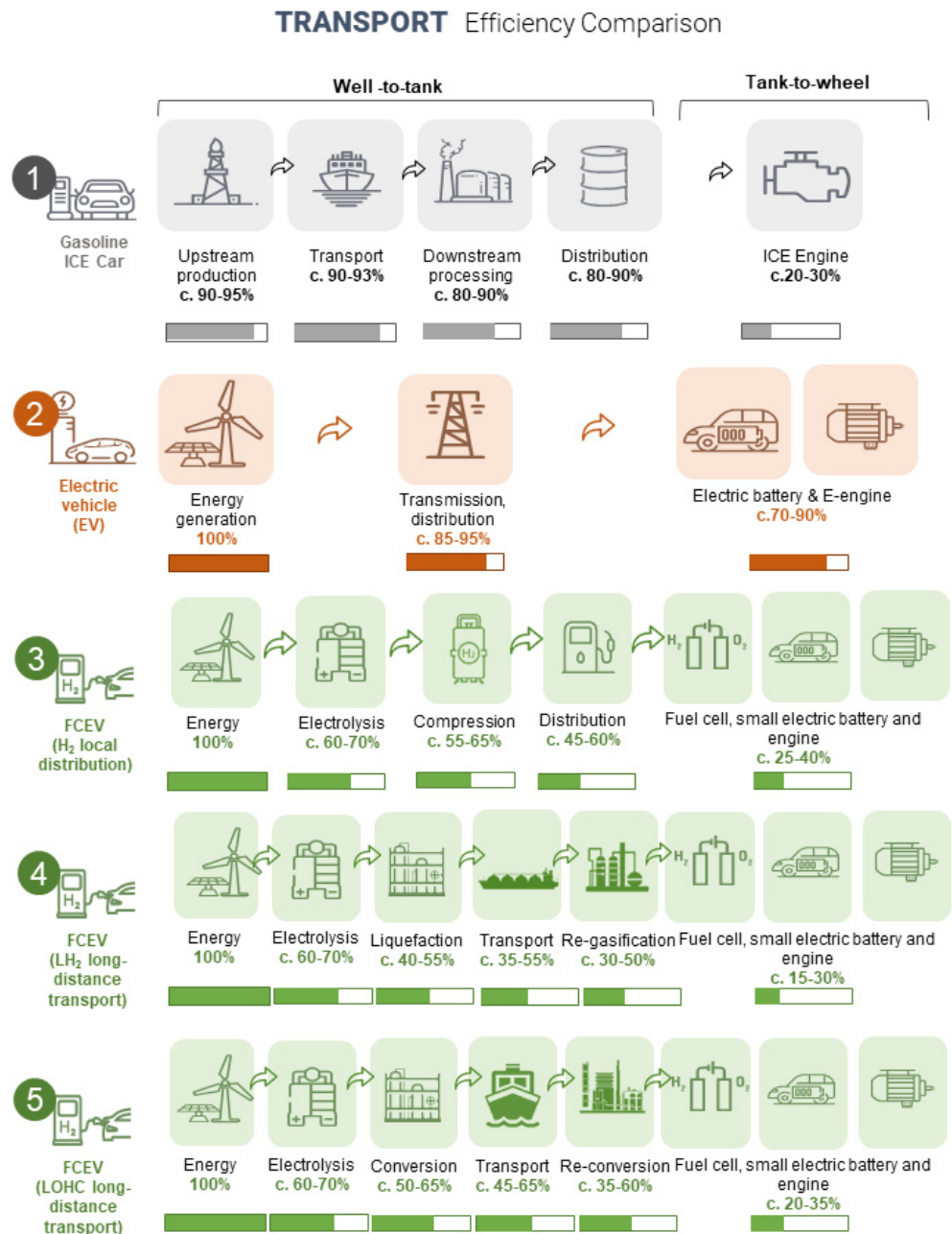
Exhibit 44: Hydrogen has a low efficiency, on a comparative basis, with electric vehicles being twice as efficient on a well-to-wheel basis
